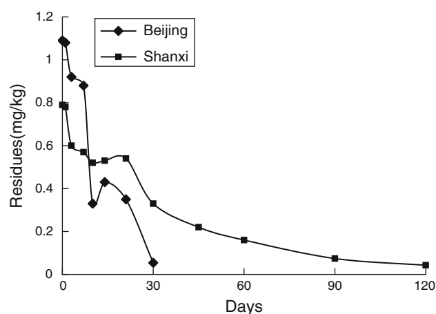
Fig. 4 Dissipation curves of residues of mefenoxam in soil
