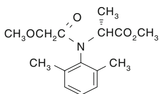
Fig. 1 Structure of mefenoxam
