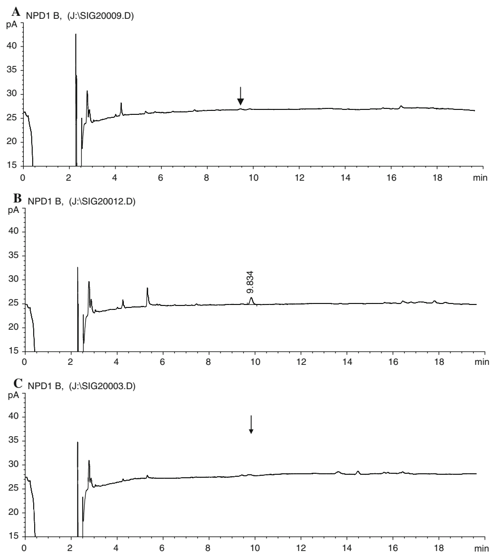
Fig. 2 Chromatograms of mefenoxam ( t_R = 9.83 ) in samples. a control (untreated whole watermelon); b spiked whole watermelon with mefenoxam working solutions at 0.05 mg/kg levels; c control (untreated watermelon flesh); d spiked watermelon flesh with mefenoxam working solutions at 0.05 mg/kg levels; e control (untreated soil); f soil (21-day sample with 0.051 mg/kg of mefenoxam); g standard (solution in methanol at 1 mg/L)
