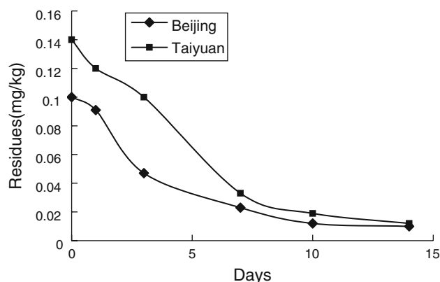
Fig. 3 Dissipation curves of residues of mefenoxam in whole watermelon
